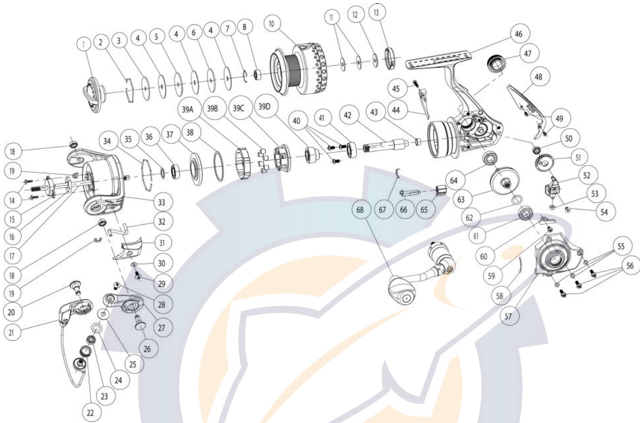
Quantum Energy E30PTIB Spinning Reel Part List
